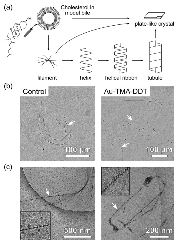
Figure 3. Amphiphilic NPs inhibit cholesterol crystallization from model bile. a) Structural evolution of cholesterol crystallization from model bile. b) OM images showing helical ribbons of cholesterol grown in the absence of the particles (left) and thin filaments stabilized by amphiphilic AuNPs (right). c) Cryo-TEM images of cholesterol filaments stabilized by Au-TMA-DDT NPs adsorbed at the edge of the filaments.
